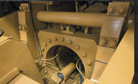
Heavy Duty Split Mainframe with Oscillating Bearing for Free Axle Pivot
